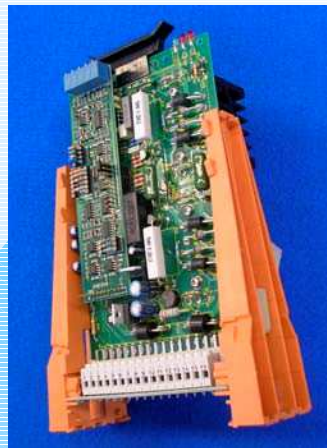
Removable calibration board with surface mounting technology (smt)
